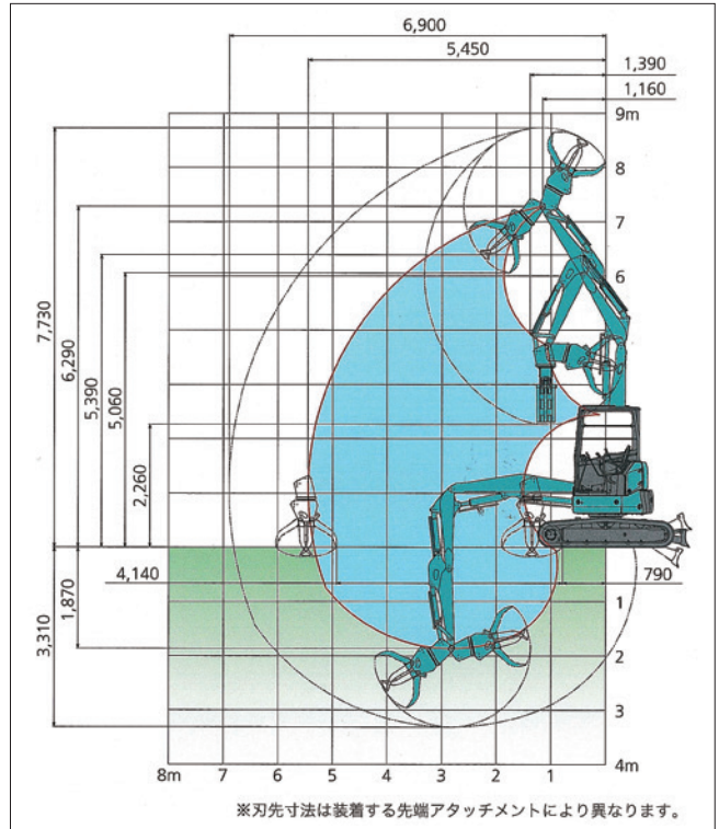
ZX35U-5B
